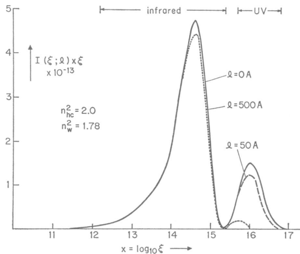
FIGURE 3 b The influence of the finite velocity of propagation on the spectrum of infrared and UV contributions to van der Waals energies. n^2_{hc} = 2.0 , data for ethane and water. Small UV contribution at l = 0 and weak dependence of A on l .
