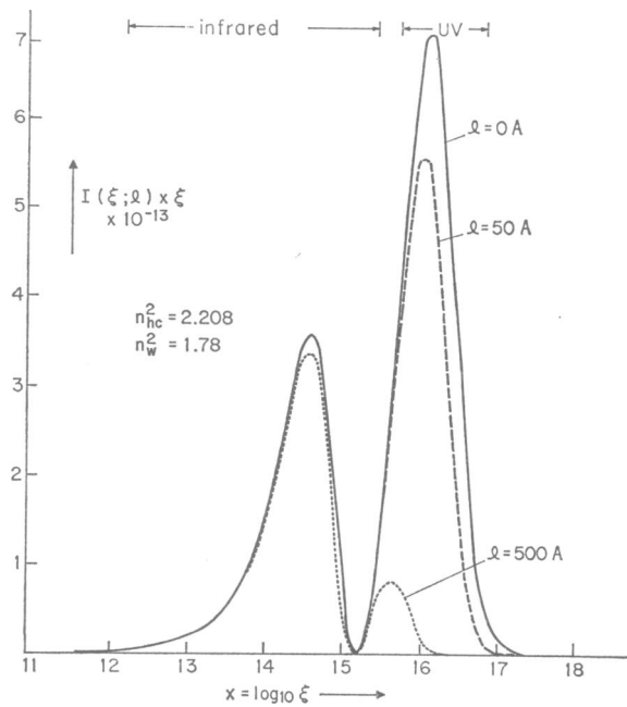
FIGURE 3 a The influence of the finite velocity of propagation on the spectrum of infrared and UV contributions to van der Waals energies. n^2_{hc} = 2.208 , data for ethane and water. Large UV contribution at l = 0 and significant decrease of A with l .
